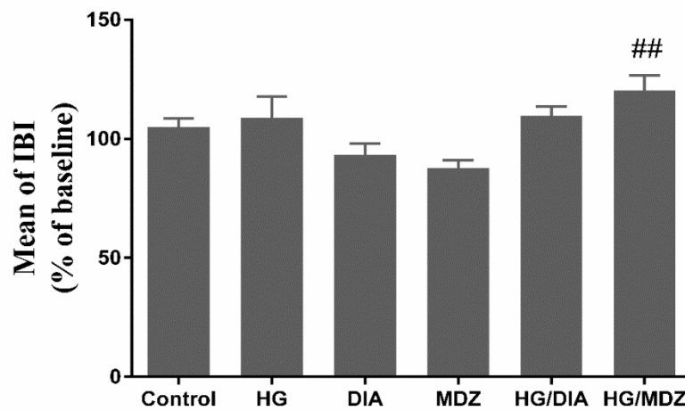
Fig.3. Mean of inter-breath interval (IBI) was analyzed by one-way ANOVA with Bonferroni post-test. ## P<0.01 compared to MDZ. Data presented as mean \pm SEM (n=7). HG: hyperglycemia, DIA; diazepam, MDZ: midazolam.
